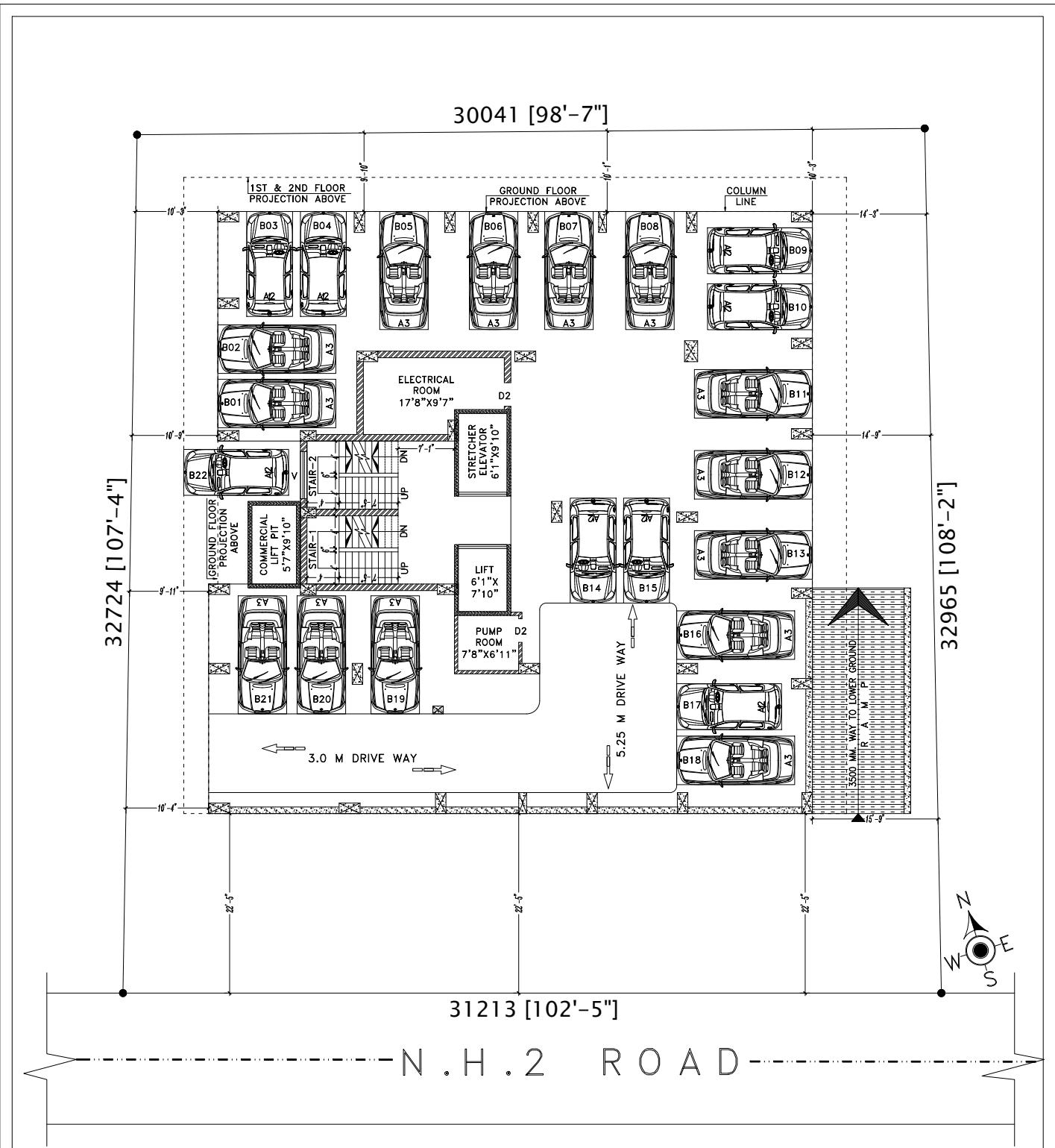
A LOWER GROUND FLOOR PLAN WITH SITE PLAN SCALE: 1:100
